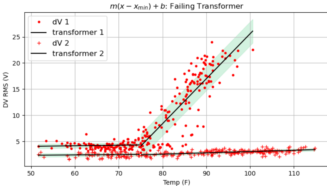
Figure 4: A scatter plot of change in voltage vs. maximum daytime temperature. This plot illustrates the difference between a transformer believed to be struggling (transformer 1) and a normal operating transformer (transformer 2).
