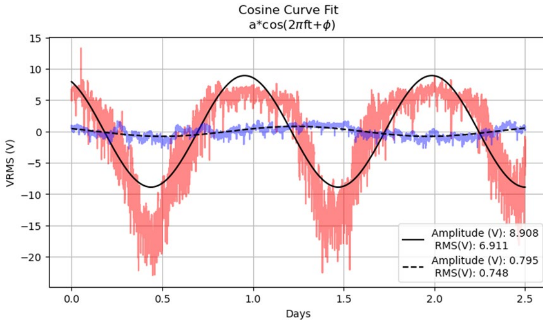
Figure 6: Voltage data from Figure 6 compared to a normal operating transformer's voltage, plotted in blue. The voltage in blue is from the same sensor as the linear comparison presented in Figure 5. Both voltages are taken from the hottest two and one-half consecutive days in August, with temperatures above or near 100 degrees. A well-behaved transformer may still show some daily sinusoidal patterns. However, when comparing the blue (normal) voltage to the red voltage of the failing transformer, the blue cosine fit possesses an amplitude value that is smaller than an order of magnitude than the red voltage's amplitude.
