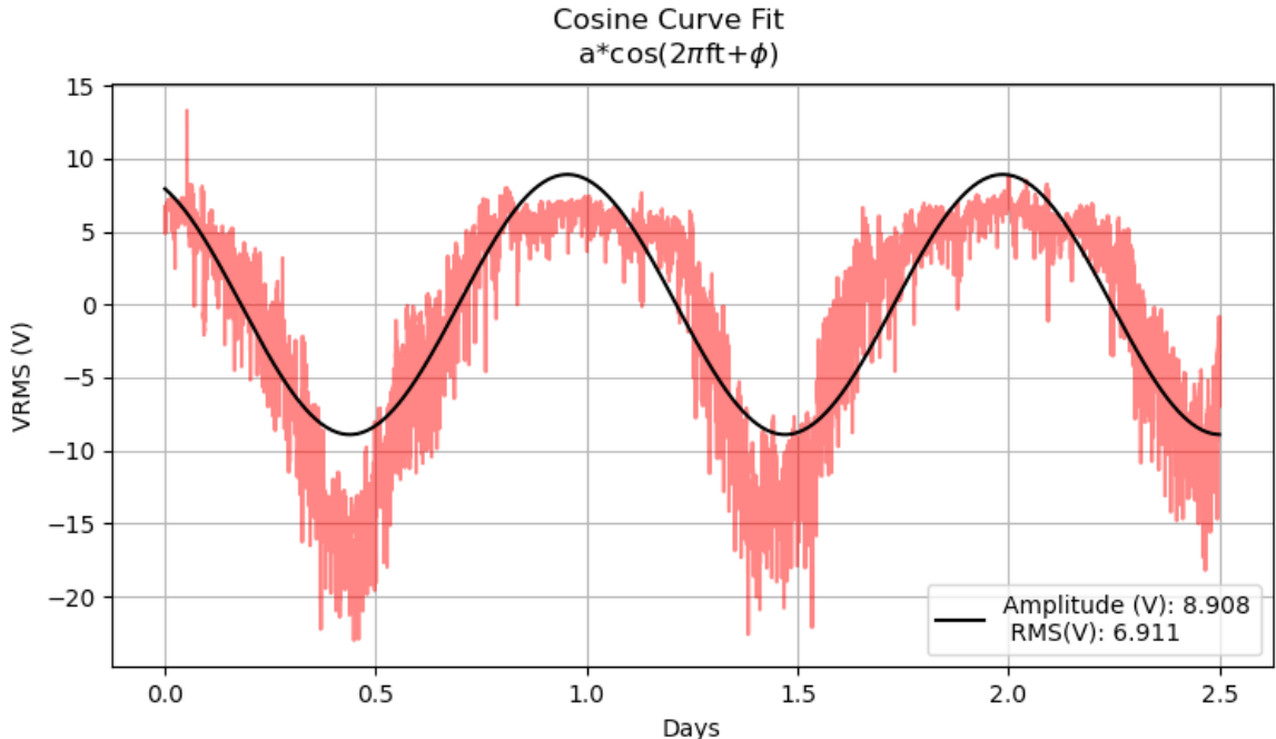
Figure 5: Two and a half days of voltage data, centered around zero, and its best-fit cosine curve. The plot shows the sinusoidal nature of a transformer dependent on the outside temperature. At t=0 the voltage data started at approximately 5 am for the homeowner's local time, therefore having the highest likelihood for cool temperatures and least load. In turn, this corresponds with a max voltage at t = 0 , or a cosine curve with little phase shift.
