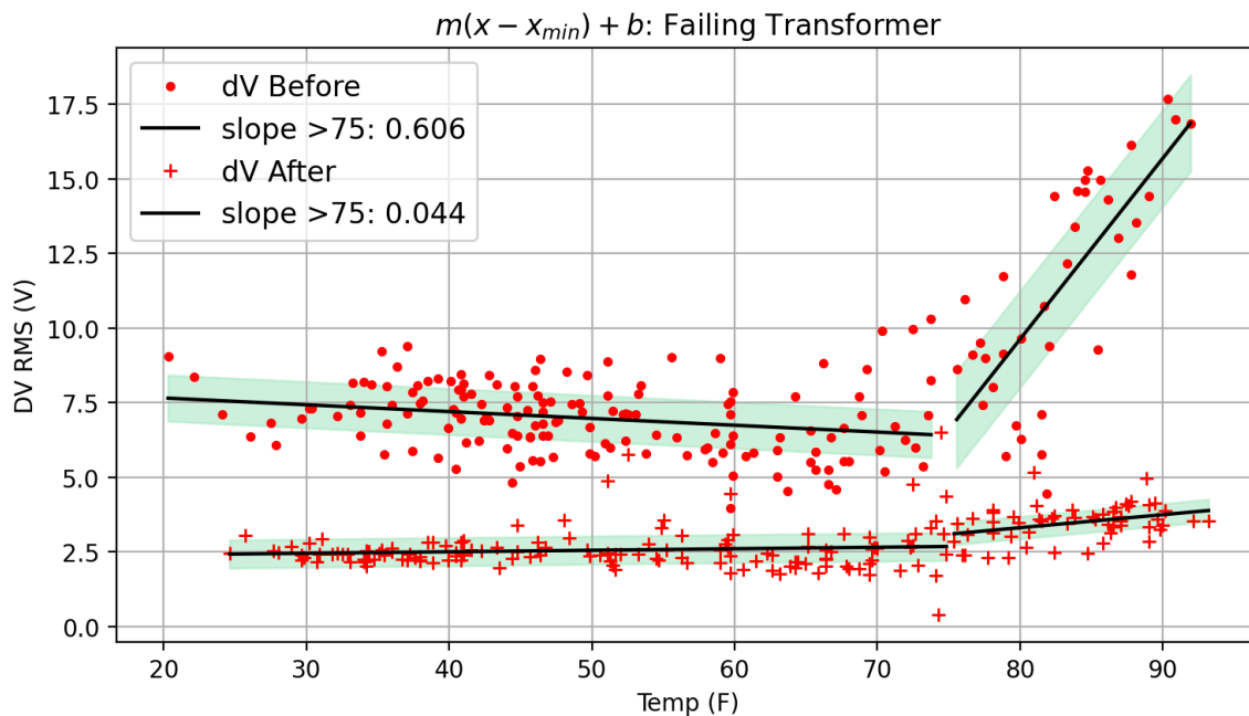
Figure 2: This scatter plot illustrates the difference in the changing voltage before and after replacing the distribution transformer serving the home. The daily change in V_{rms} is plotted on the y-axis, with the daily high temperature on the x-axis. The circular points illustrate the change in voltage for a given daily high temperature before transformer replacement, while the "+" points indicate the same data after replacement. This plot shows a correlation between the maximum daytime temperature and the voltage change for an overloaded transformer.
